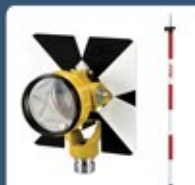
PRISM ROD WITH TARGET PLATE
